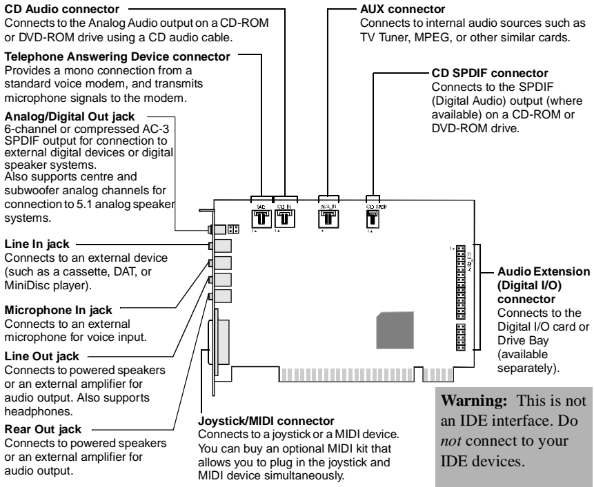
Jacks and connectors on the SB Live! Player 5.1 card.
